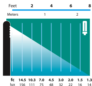
PL-07-FL-7 Light Distribution and Photometrics 8 ft. (2.4m) radius
